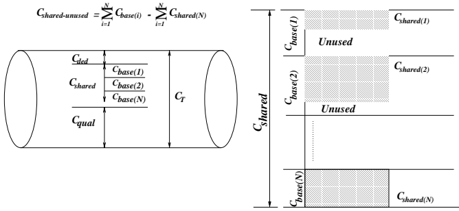
Fig. 5. Microscopic View of Bandwidth Apportionment at Edge
