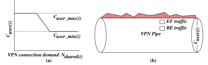
Fig. 3. The SLA approach: (a) Bandwidth is specified as an interval of C_{user\_min(i)} and C_{user\_max(i)} for any group i . Actual rate of a VPN connection C_{user(i)} varies between this range but never gets below C_{user\_min(i)} . (b) C_{user(i)} is the rate that is configured in the edge router as the policing rate. Traffic submitted at a rate higher than this rate is marked as best effort traffic or dropped depending on the policy
