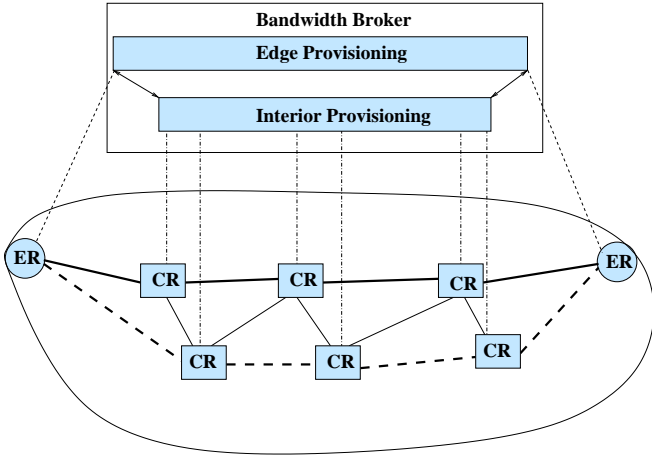
Fig. 2. Layered Provisioning view of VPN-Diffserv Networks
