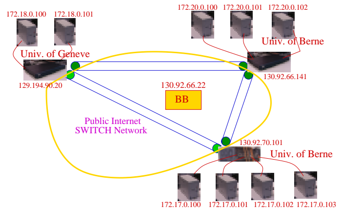
Fig. 7. Experimental Setup of VPN
